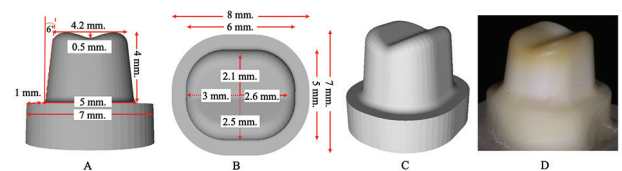
Figure 2: The abutment was designed on a computer using SolidWorks software. (A) Dimensions of the abutment in the proximal view; (B) Dimensions of the abutment in the occlusal view; (C) A 3D design of the abutment was created; (D) The abutment was milled from a 3D design using a milling machine.
